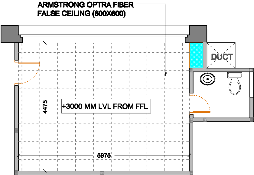
REFLECTED CEILING PLAN LAYOUT
