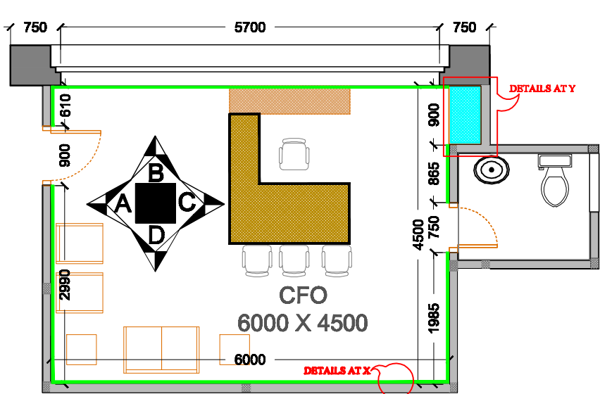
FURNITURE LAYOUT PLAN
